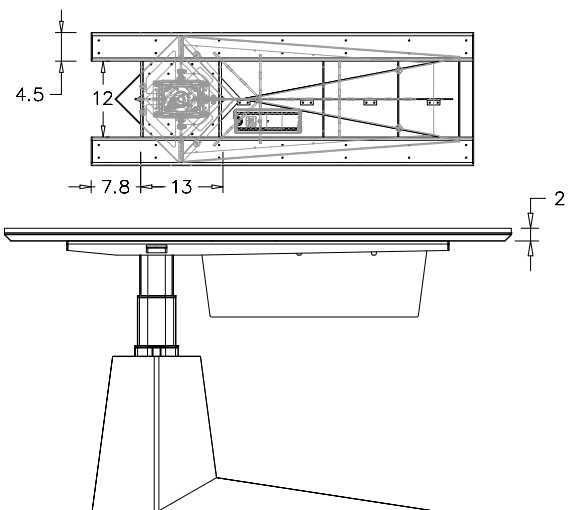
FRAME OPENING DIMENSIONS (SAME FOR ALL TABLE SIZES)
