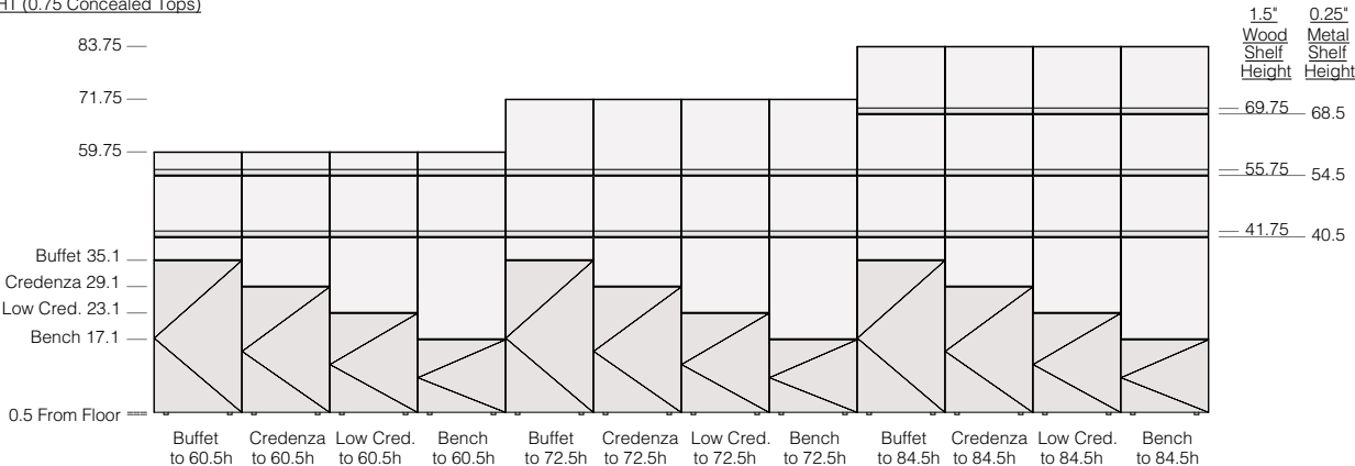
CADENCE HEIGHT (0.75 Concealed Tops)
