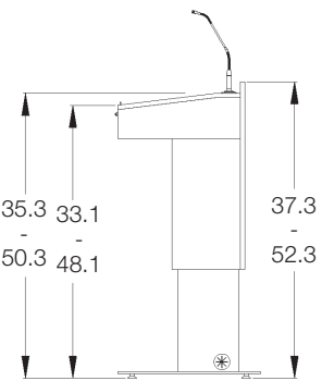
Height Adjustable/Non-Mobile
