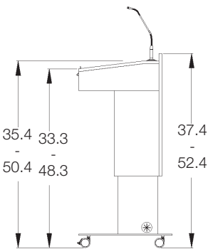
Height Adjustable/Mobile
