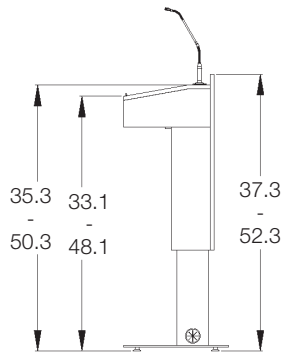
Height Adjustable/Non-Mobile
